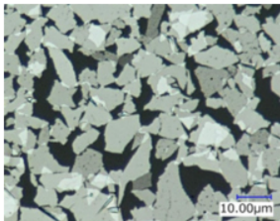
Flake shape
